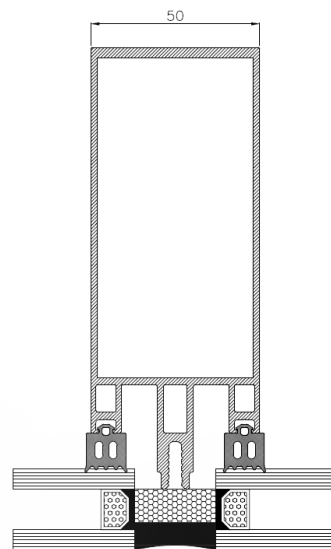
Upright section
