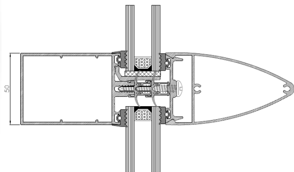
Transom section
