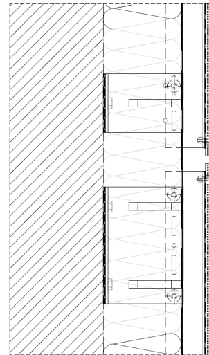
Horizontal section.
